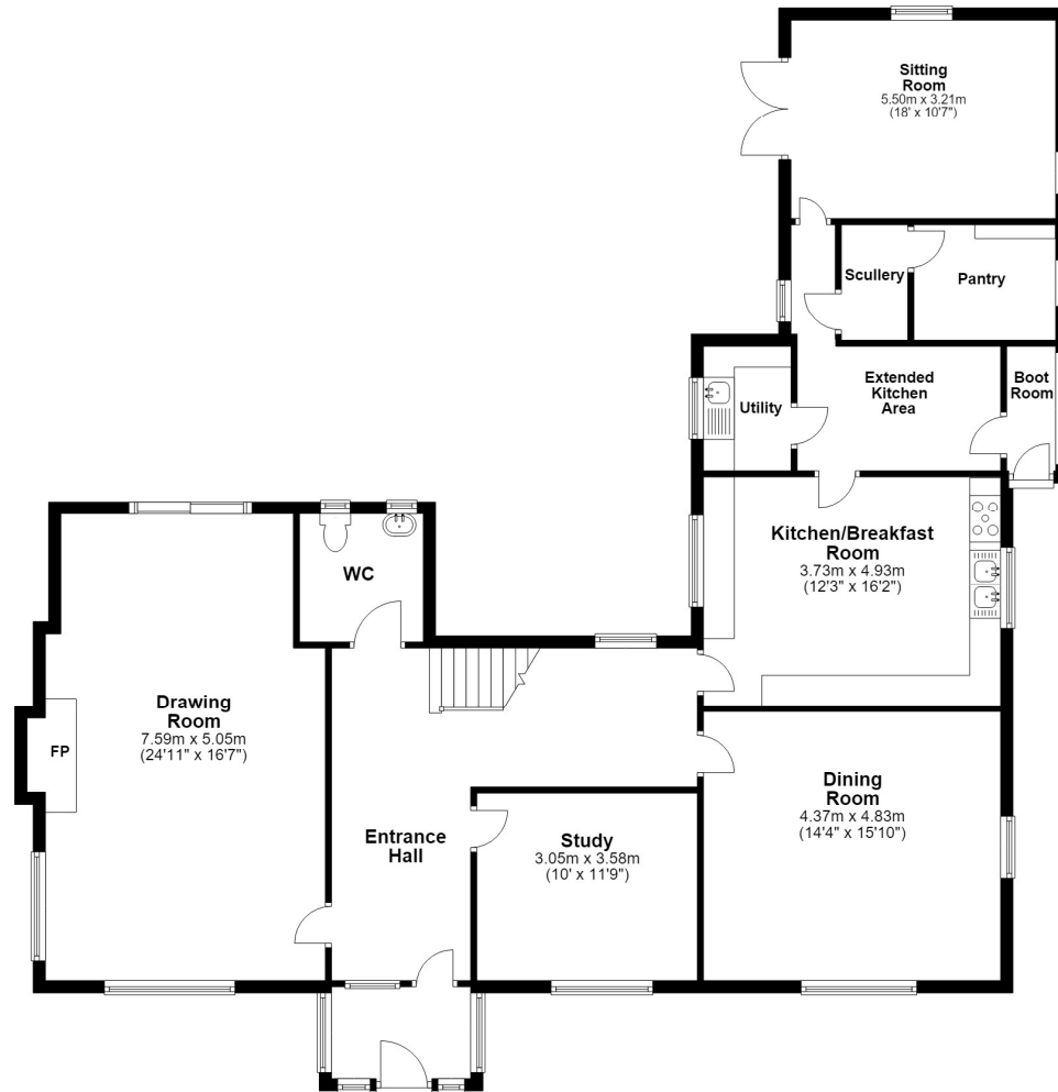
Ground Floor
